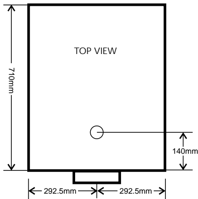
BELVEDERE 5000 TOP & BACK VIEW hydronic heating
